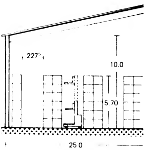
12 Use of storage space with fork-lift
